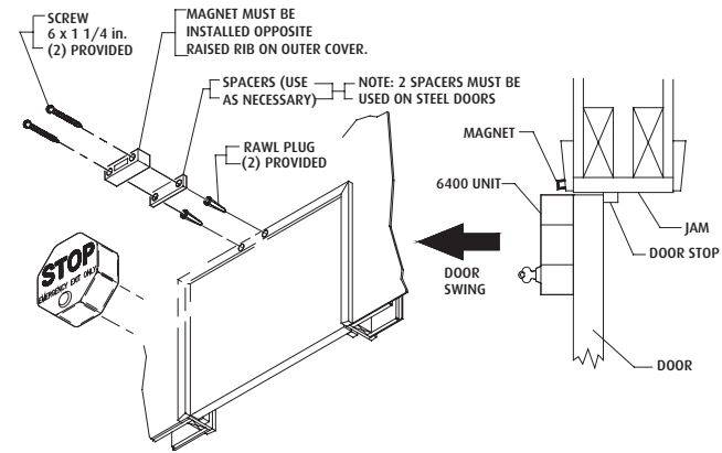
TYPICAL FLUSH MOUNT DOOR JAM INSTALLATION
