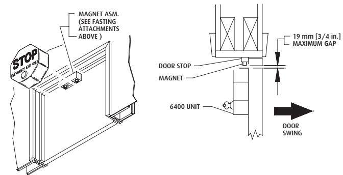
TYPICAL DOUBLE DOOR INSTALLATION STI 6402
